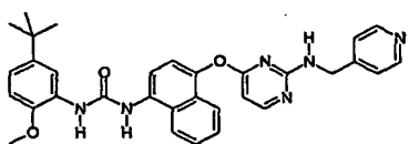
1-(5-tert-Butyl-2-methoxy-phenyl)-3-(4-{2-[(pyridin-4-ylmethyl)amino]-pyrimidin-4-yloxy}-naphthalen-1-yl)-urea;
